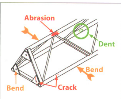
Steel Truss
