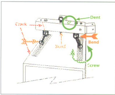
Loudspeaker Rigging
