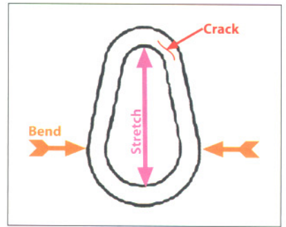
Pear Ring
