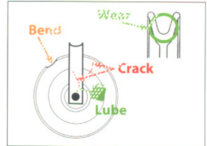
Sheave
